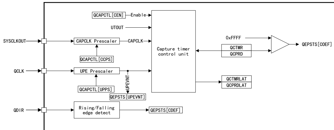
Figure 186 Structure Block Diagram of Edge Capture Unit
