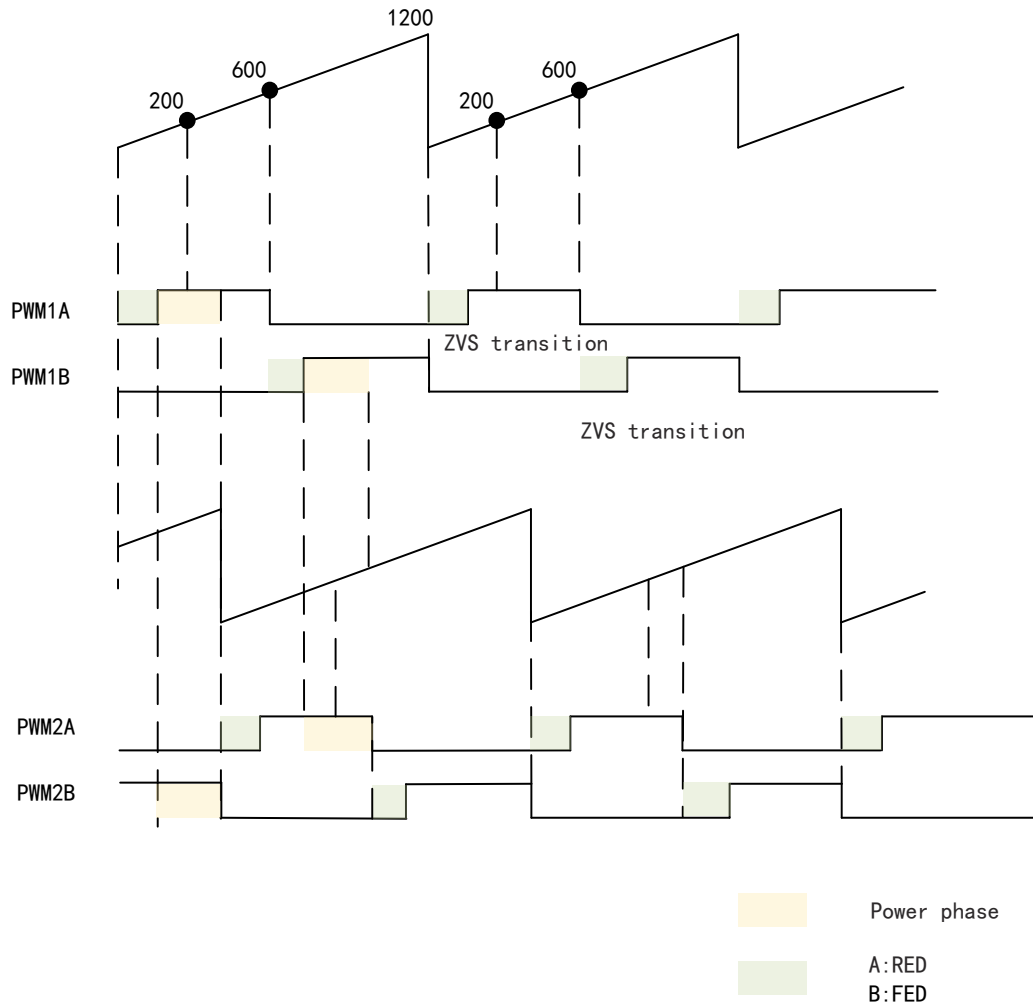
Figure 137 Full H-bridge Waveform Diagram
