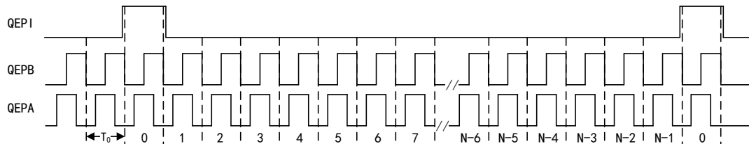
Figure 168 QEP Encoder Output Signal in Counterclockwise Rotation
