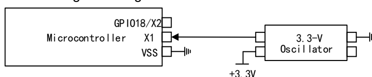
Figure 5 Single-ended 3.3V External Clock
