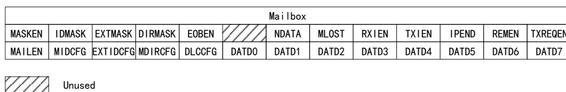
Figure 252 Mailbox Structure
