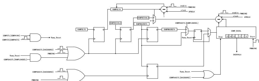
Figure 56 Ramp Generator
