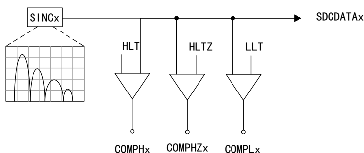
Figure 70 Comparator Unit Structure
