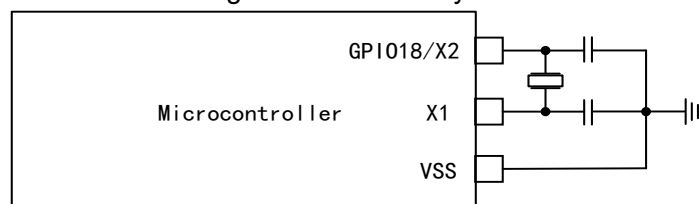
Figure 6 External Crystal
