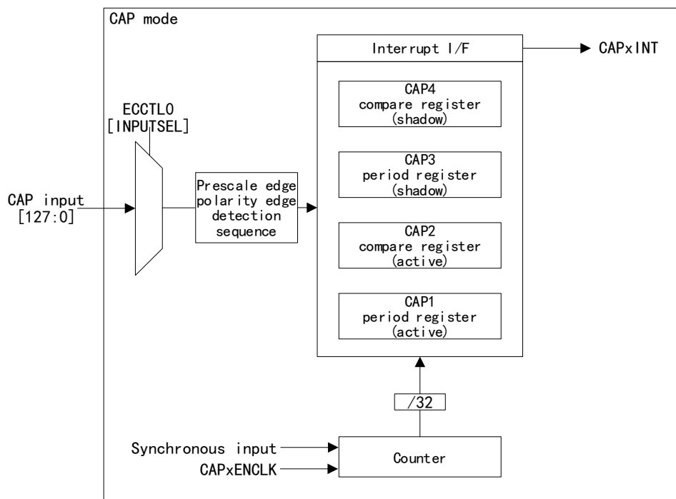
Figure 148 CAP Mode Structure Block Diagram
