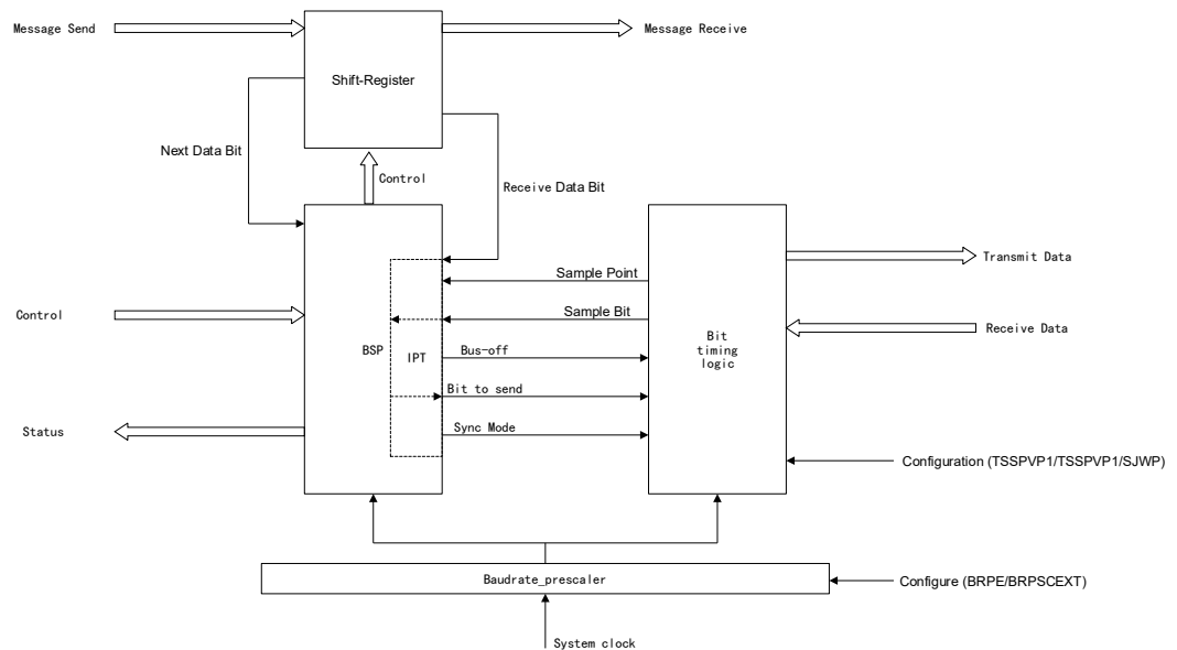
Figure 257 CAN Protocol Controller Structure
