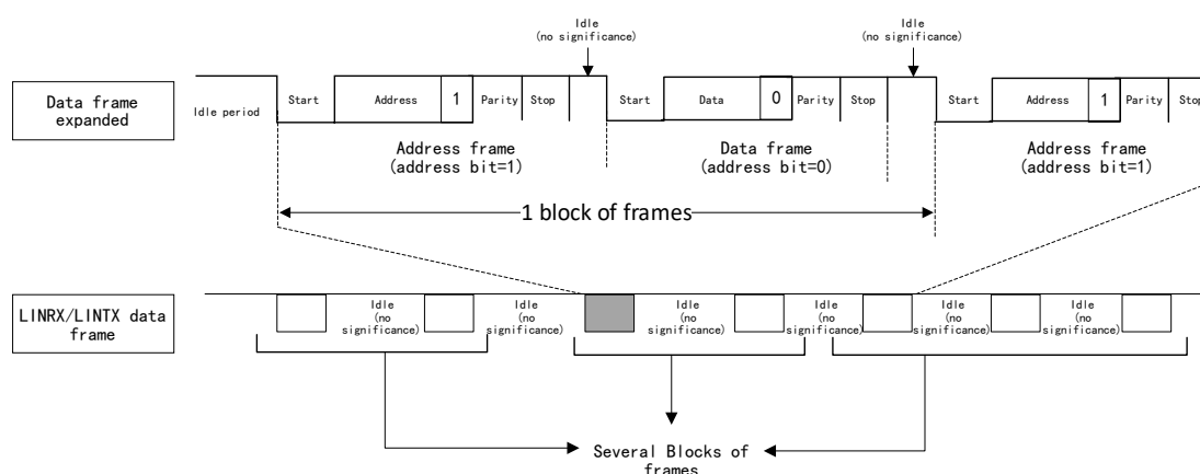
Figure 281 Address Bit Multiprocessor Communication Format
