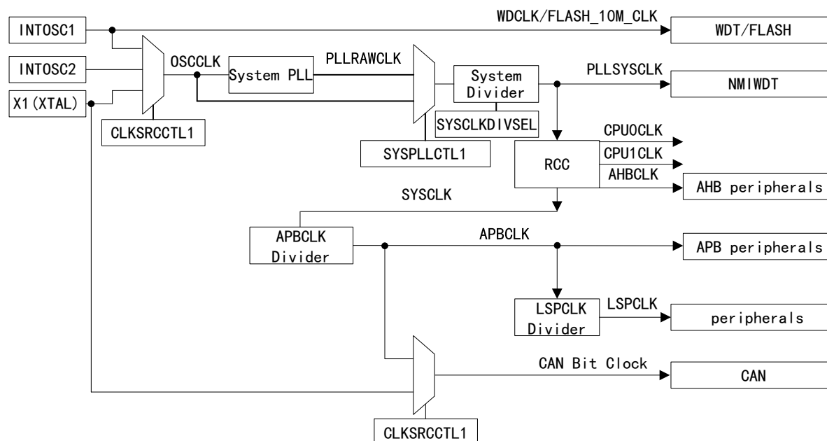
Figure 3 Clock Source
