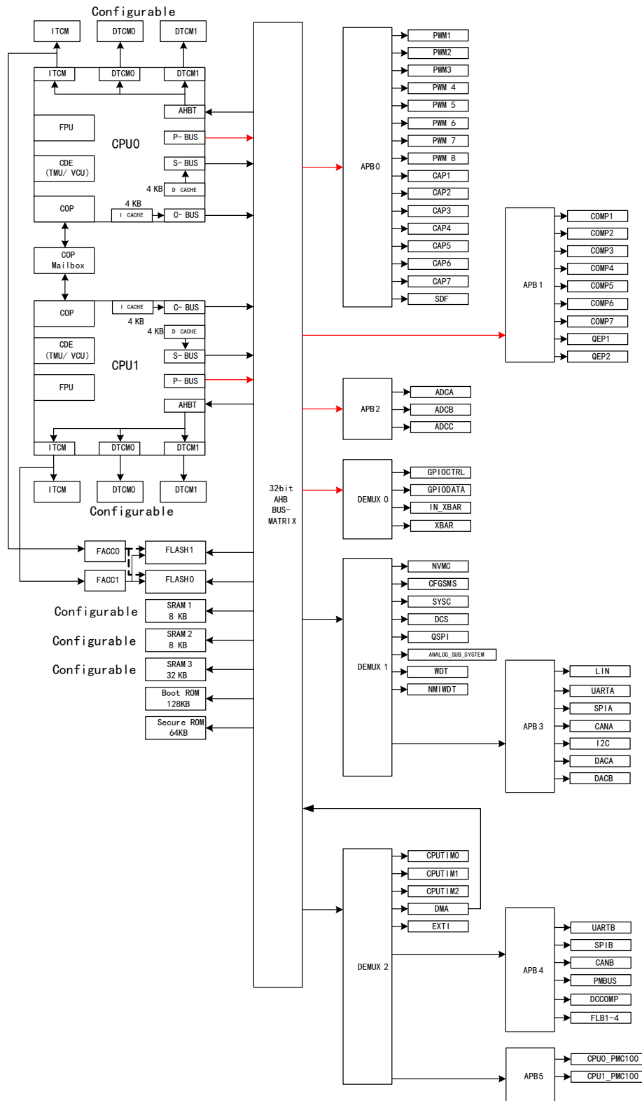
Figure 1 CPU Architecture
