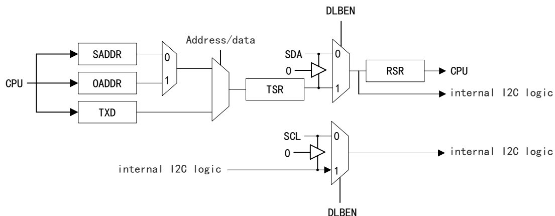
Figure 213 Digital Loopback Mode
