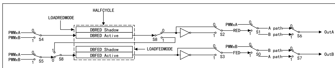
Figure 102 Structure Block Diagram of Dead-band Generator Submodule
