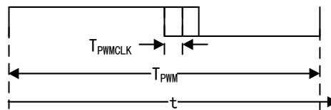
Figure 141 Timing Diagram of a Conventionally Generated PWM
