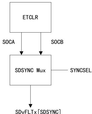
Figure 69 SDSYNC Event
