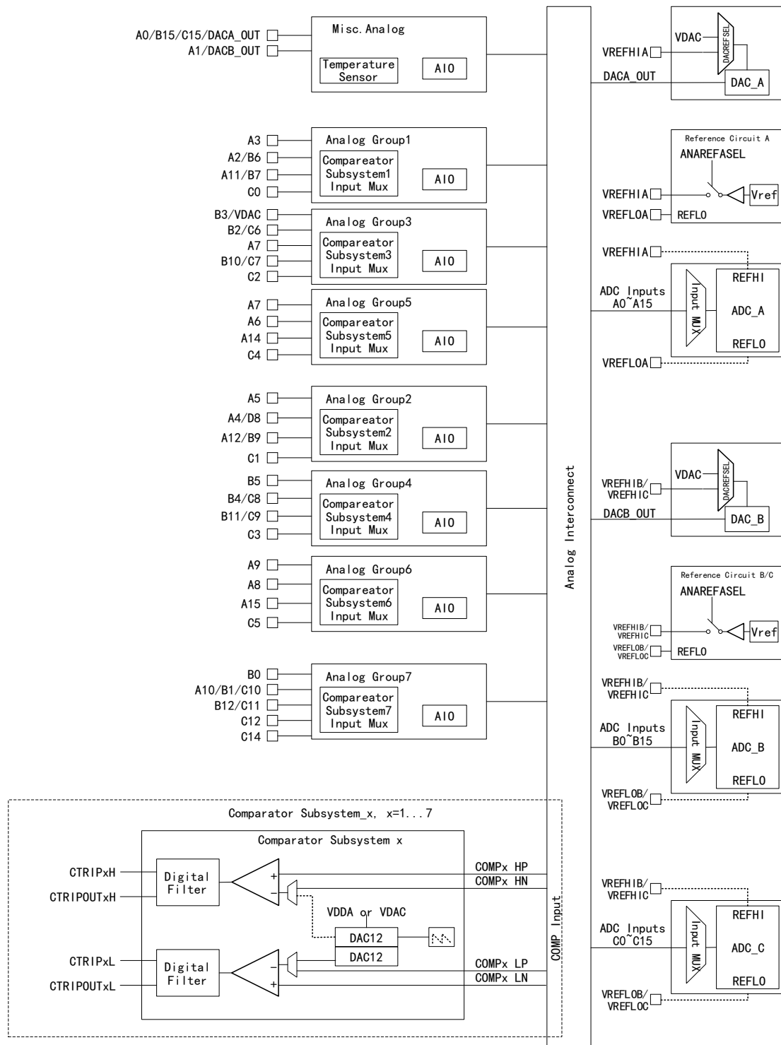
Figure 39 Analog Subsystem Block Diagram (100-pin)
