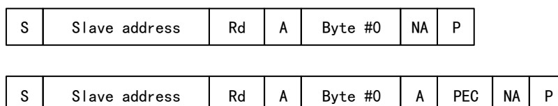
Figure 232 Receive Byte Message with and without PEC
