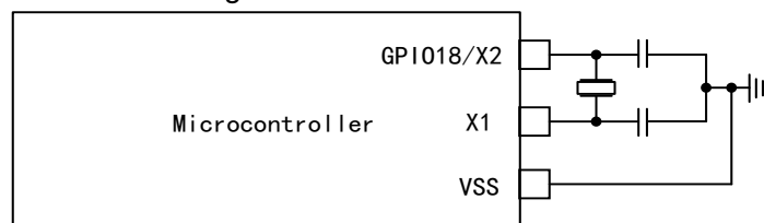
Figure 7 External Resonator
