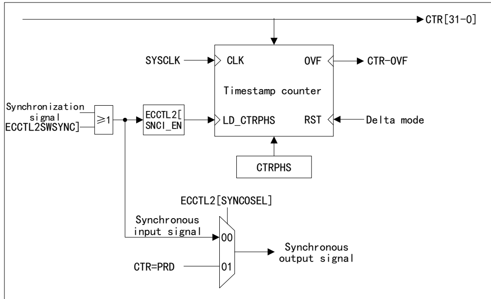
Figure 152 Counter and Synchronization Function Structure Block Diagram
