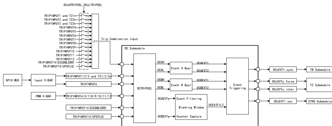
Figure 114 Structure Block Diagram of Digital Compare Submodule
