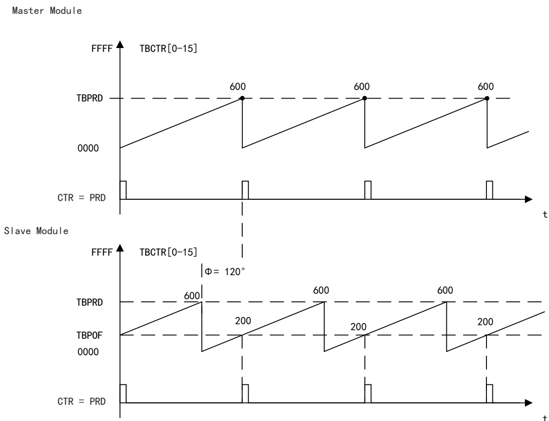
Figure 135 Waveform Diagram for Phase Synchronization between Two PWM Modules
