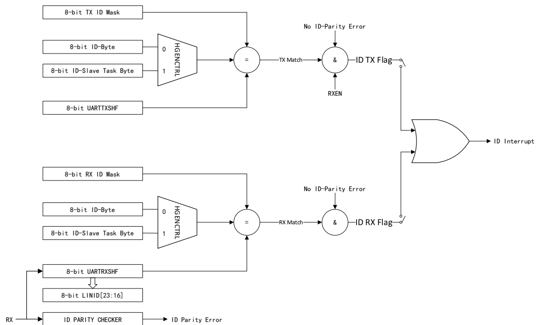
Figure 274 ID Reception Filtering, and Validation
