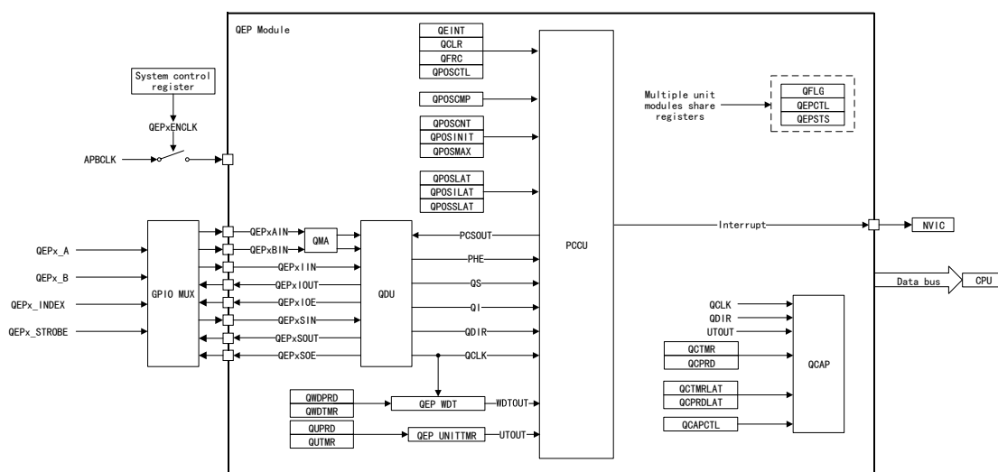
Figure 165 QEP Structure Block Diagram
