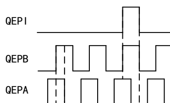
Figure 166 QEPI Waveform Diagram
