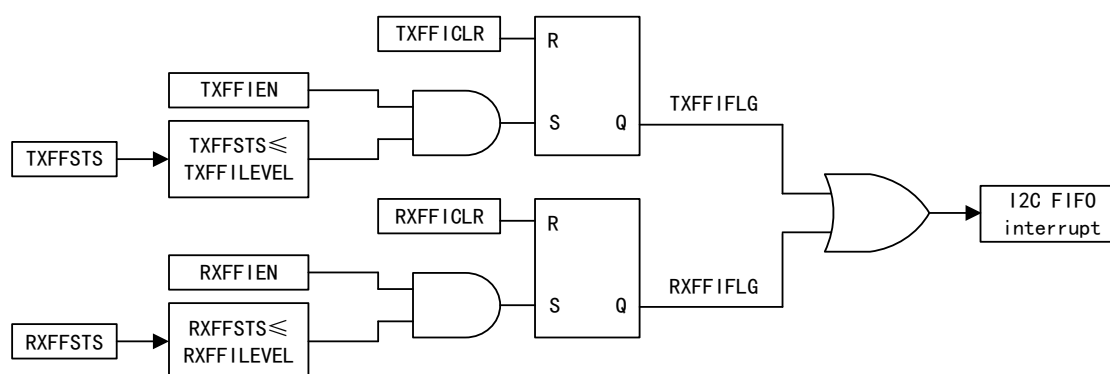
Figure 216 FIFO Interrupt
