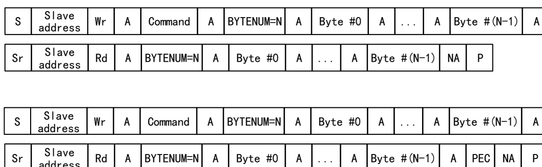
Figure 229 Block Write with or without PEC - Block Read Process Call Message
