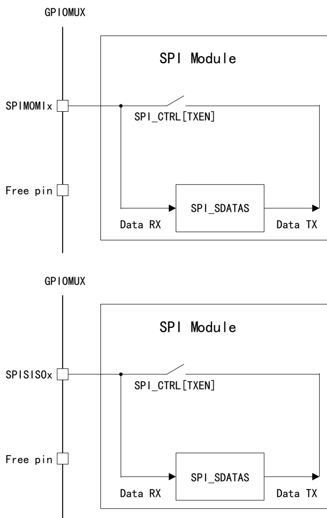
Figure 198 SPI 3-wire mode
