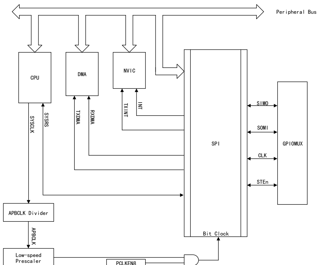
Figure 189 CPU Interface Structure Block Diagram of SPI
