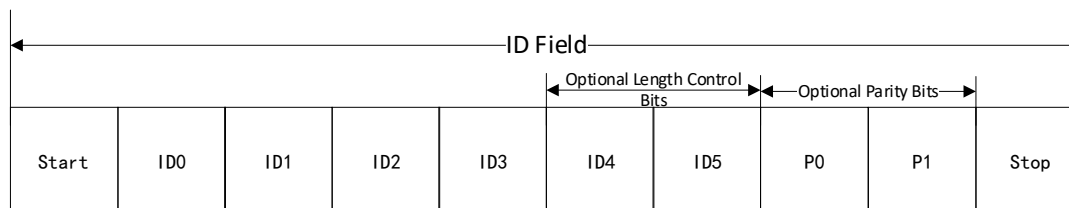
Figure 269 ID Field
