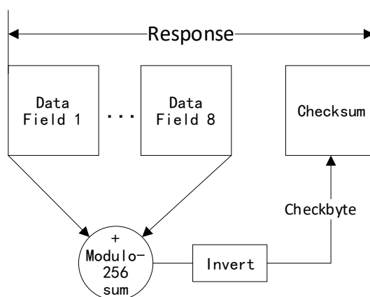
Figure 273 LIN 2.0 Compatible Checksum Generation for Transmitting Nodes
