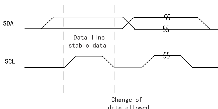
Figure 210 Data Validity
