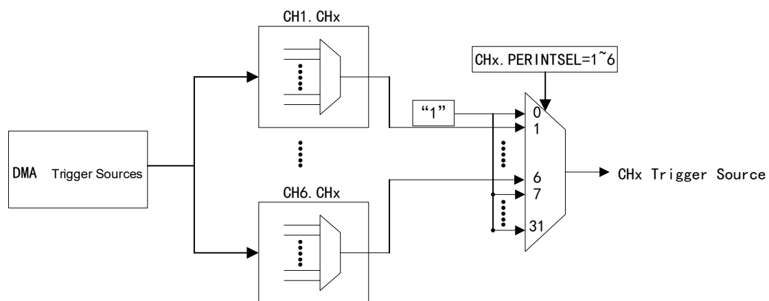
Figure 27 DMA Trigger Structure
