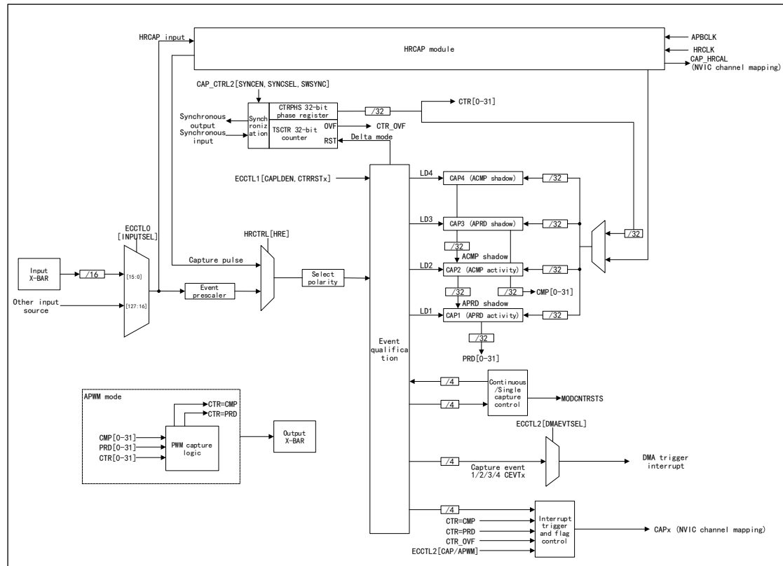
Figure 147 CAP Structure Block Diagram
