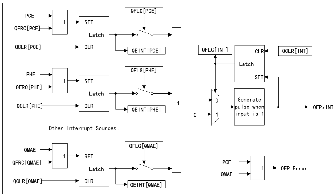
Figure 172 QEP Interrupt Structure Block Diagram
