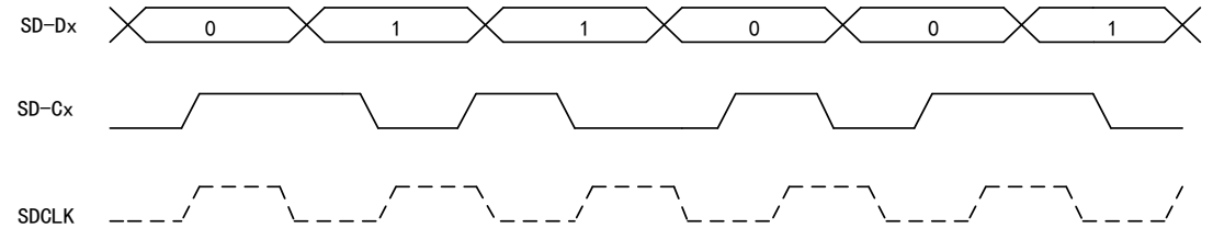
Figure 64 Operation in Modulator Mode 2
