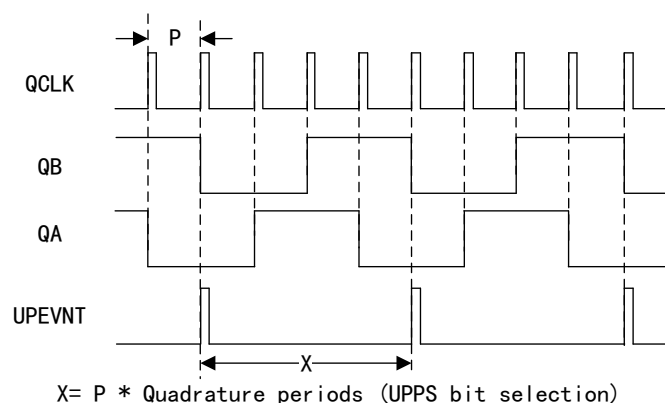
Figure 187 Timing Diagram of Unit Position Event
