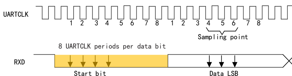
Figure 203 Asynchronous Communication Format
