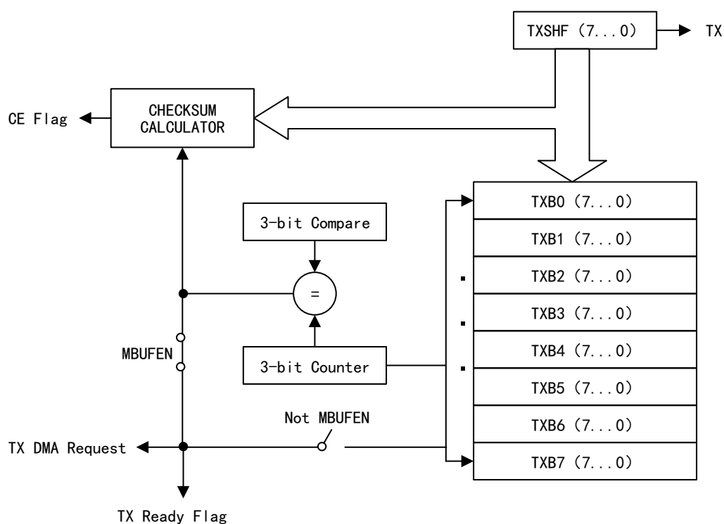
Figure 283 Transmit Buffer
