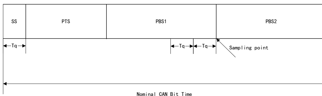
Figure 253 Bit Timing
